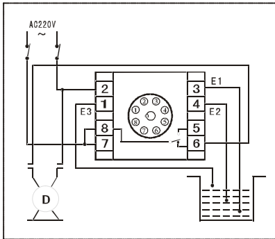
(供水接线图 Water supply wiring diagram)
