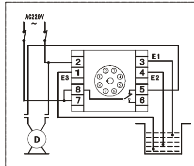
(排水接线图 Draining water wiring diagram)
