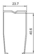
ARS-H10A (钢制卡簧)
